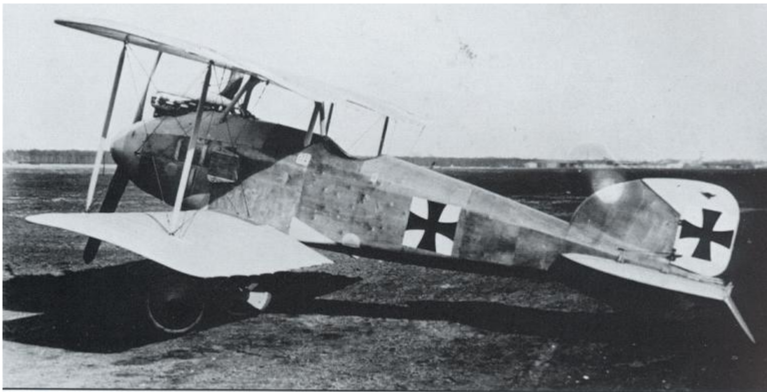
Dipl.-Ing. Thelan's new design, the Albatros D. I. The Albatros company logo can be seen just above the rudder cross.
